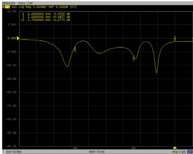
Reference measurement in a non-reflective environment, without DUT or other mechanics in surrounding area
